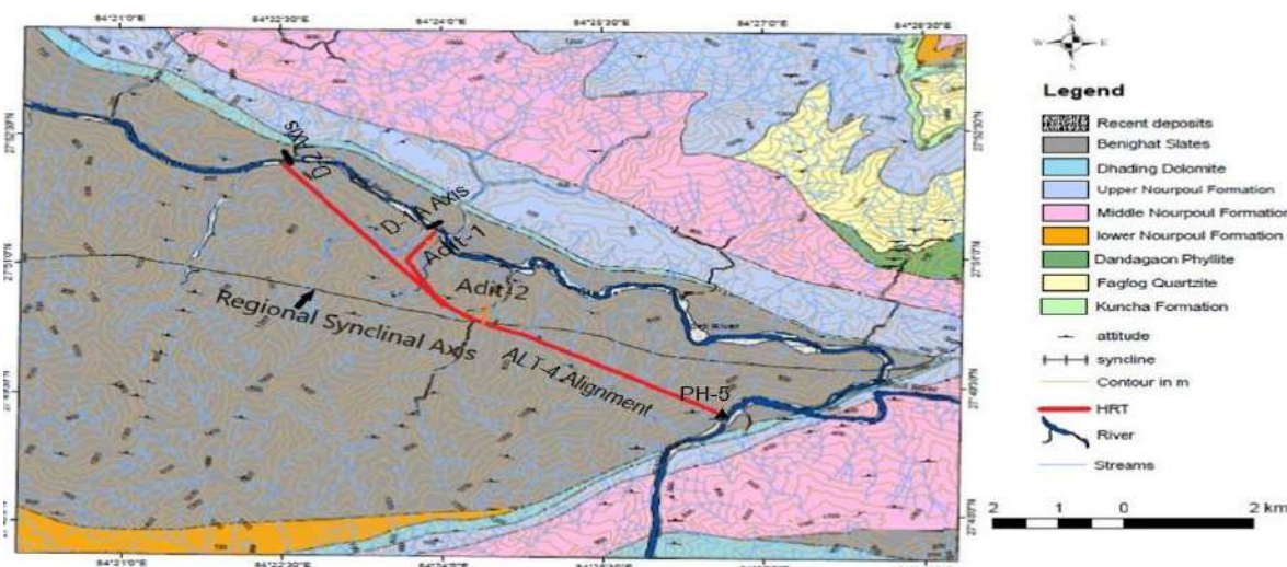
Figure 31: Regional geology of the project area (DMG, GON)
