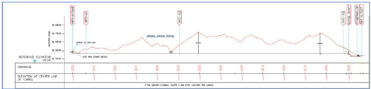
Figure 80: Longitudinal Profile of HRT Alternative 4
